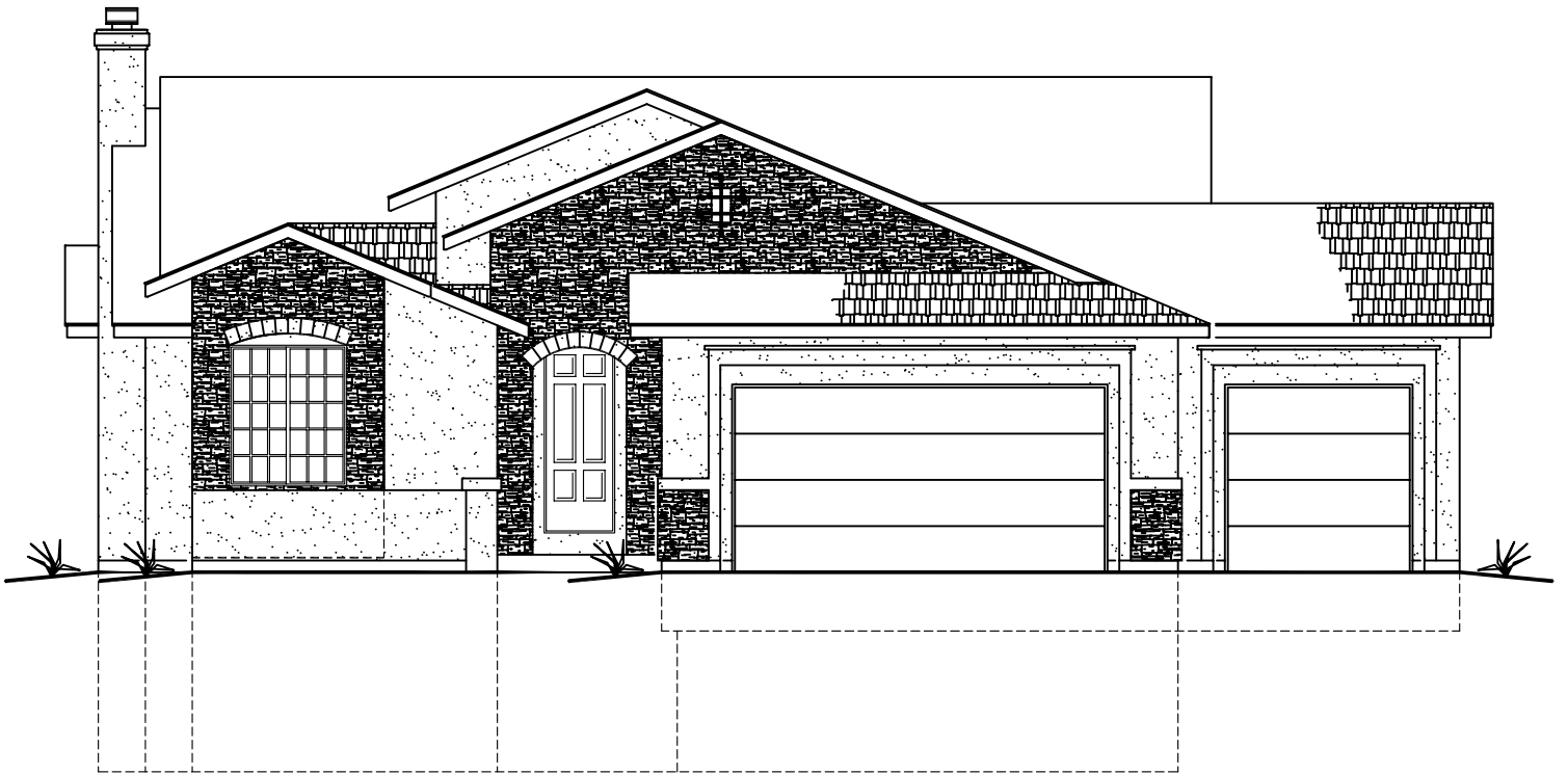
FRONT ELEVATION
