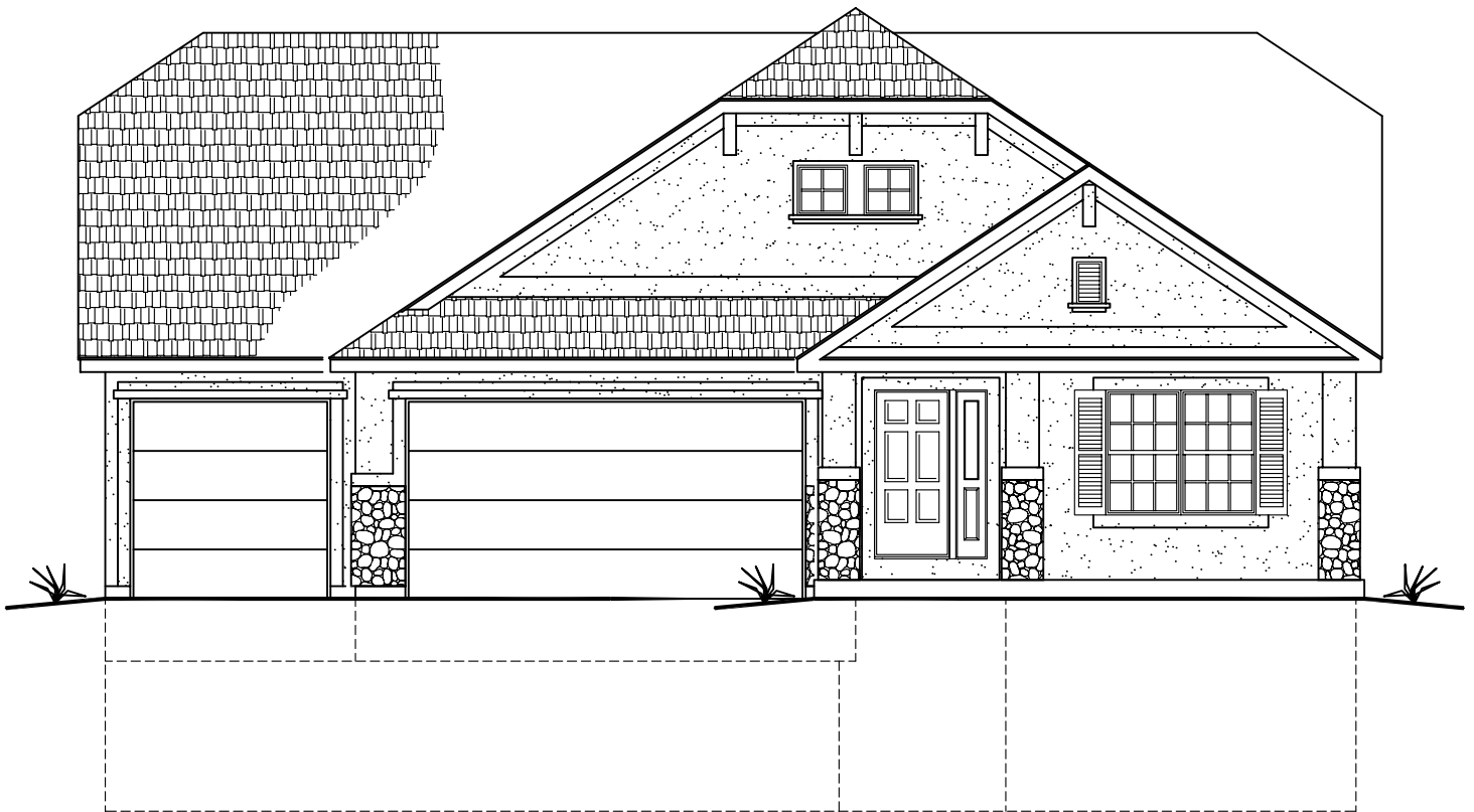
EUROPEAN COTTAGE FRONT ELEVATION
