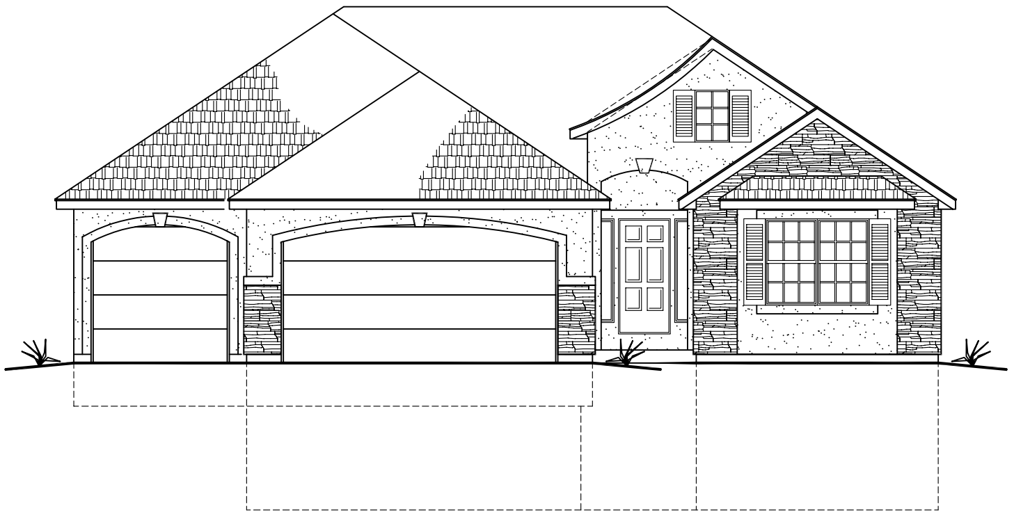
FRENCH COUNTRY FRONT ELEVATION
